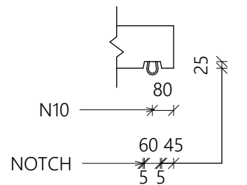
NOTCH DETAIL-A
