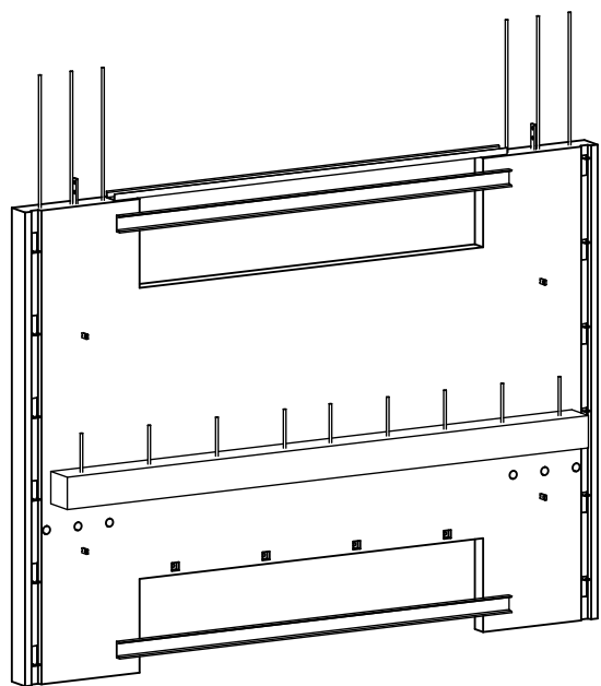
6 3D VIEW
